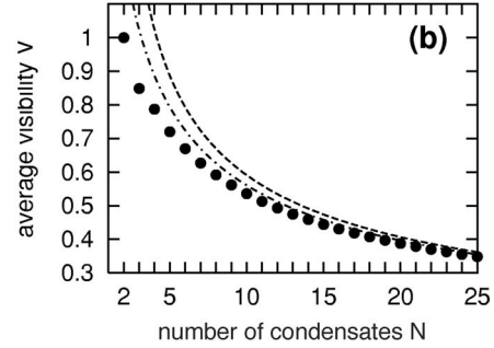
FIG. 1. (a) Random walk of coefficients z_q = e^{i\Delta\theta_q} , with the phase angles 0 \leq \Delta\theta_q < 2\pi arbitrary in the complex plane. The vector z is the sum of N-1 independent coefficients z_q ( 1 \leq q \leq N-1 ) and determines both the fringe visibility V = 2S/N with S = |z| and its phase angle \varphi . (b) Predicted average fringe visibility for the far-field interference pattern of N coherent atomic sources (dots). Result of the central limit approximation: V = \sqrt{\pi}/(N-1) (dashed line) and the simple V = \sqrt{\pi}/N scaling function (dashed-dotted line).
