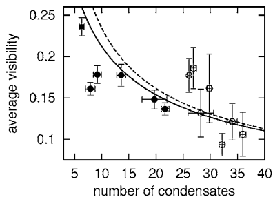
FIG. 3. Average fringe visibilities of far-field interference patterns as a function of number of interfering coherent atomic sources. The experimental data sets were recorded with beam waists: 24.3 \mu\text{m} (squares), 30.0 \mu\text{m} (dots), and 40.2 \mu\text{m} (circles). The data have been fitted with the (interpolated) theoretical fringe contrast multiplied by a constant factor, which is left as a free parameter to account for the finite imaging resolution (solid line). The dashed line gives the corresponding result in the central limit approximation when assuming the same imaging resolution.
