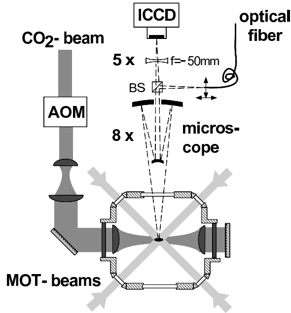
Figure 19.3: Schematic of the experimental apparatus.
