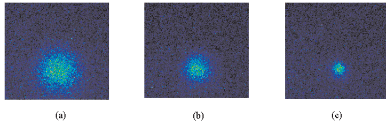
Figure 19.5: Images of the crossed dipole trap after 15 ms expansion. The phase space density (psd) has been calculated by measuring the trap vibrational frequencies, the atomic temperatures and the number of atoms remaining in the trap for different final potential depths. (a) Before forced evaporation; psd: 1/200. (b) During forced evaporation; psd: 1/60. (c) After evaporation; psd: 1/15.
