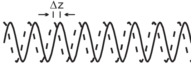
Figure 19.1: Spatial intensity dependence of two 1D standing-waves with \sigma^+ (solid), \sigma^- (dashed) respectively circular polarization. The two standing-waves are spatially shifted relative to each other by \Delta z . For a suitable laser detuning, atoms in the ground-state level |g+\rangle are pulled into the intensity maxima of the \sigma^+ -polarized standing-wave, whereas atoms in the |g-\rangle state are trapped in the maxima of the \sigma^- -polarized standing-wave.
