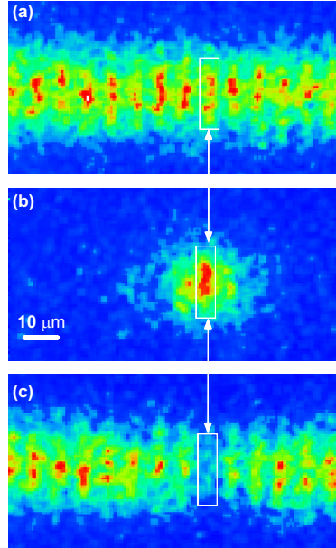
Figure 19.4: Images of the lattice after the following manipulations: (a) No manipulation of the atoms in the micro-traps. (b) Only atoms from a single lattice site are illuminated during the exposure with a focused laser beam. (c) Image of the lattice after removing atoms in one lattice site before the exposure.
